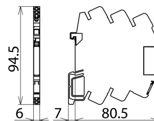
Dimension drawing DCO SD2 ME 24
