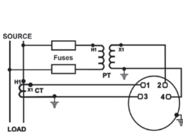
Fig. A1 Models 007-215, 078-215 Wattmeter single phase
