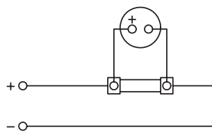
DC amps - for use with external shunt
